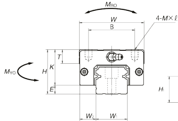
Front view of AL and BL types
