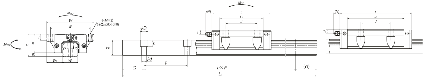
Front view of EM and GM types
