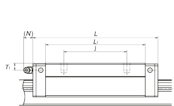
Side view of BL type
