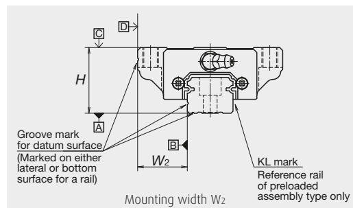
Fig. 3 Specifications of accuracy
